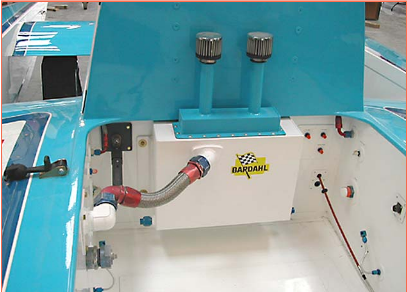
The forward engine bay with bulkhead pressure fittings, throttle and mixture cables and the Ron Brown engineered oil sump/vent tank. The six-pin cannon plug and fuel fittings can also be seen to the far right.
